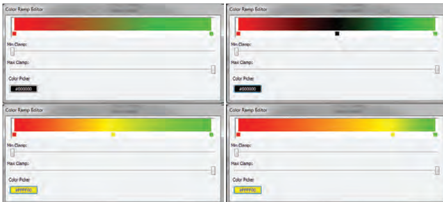
Fig. 13. Some images from an interactive session with the color map editor. The top-left image shows the initial state of the editor. The top right image shows the result when the user inserts a new sample (black) in the center of the color map. The bottom-left image shows the result after the user has updated the color of the middle sample to yellow. Finally the bottom-right image shows the effect that dragging the middle sample to right has. The color values between each sample are constructed using interpolation.
