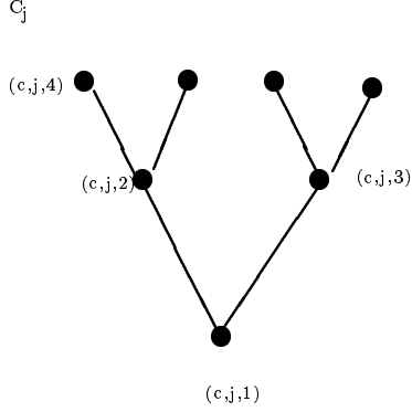
Figure 4: Local view of Tseitin graphs for C_j 's
