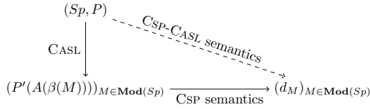
Fig. 2. CSP-CASL semantics.
