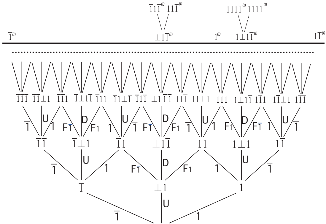
Fig. 2. The domain RD and constructors of pre-Gray code. Here, \text{LR}_{-1} , \text{LR}_1 , U , \text{Fin}_{-1} , \text{Fin}_1 , and D are written as \bar{1} , 1 , U , F\bar{1} , F1 , and D , respectively.
