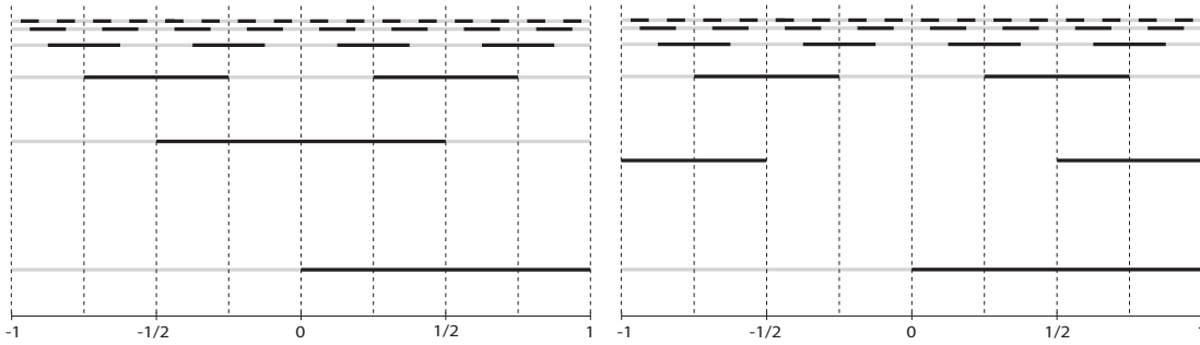
Fig. 3. Expansion by G (i.e., Gray expansion) and expansion by H.
